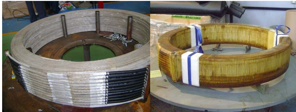
Figure 3. Field Coil
