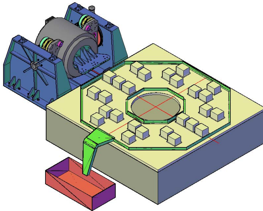
Figure 6. Overall Configuration of Shaker Slip Table System
