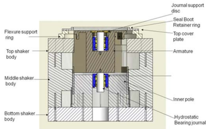
Figure 1. Cross-section view of electrodynamic shaker
